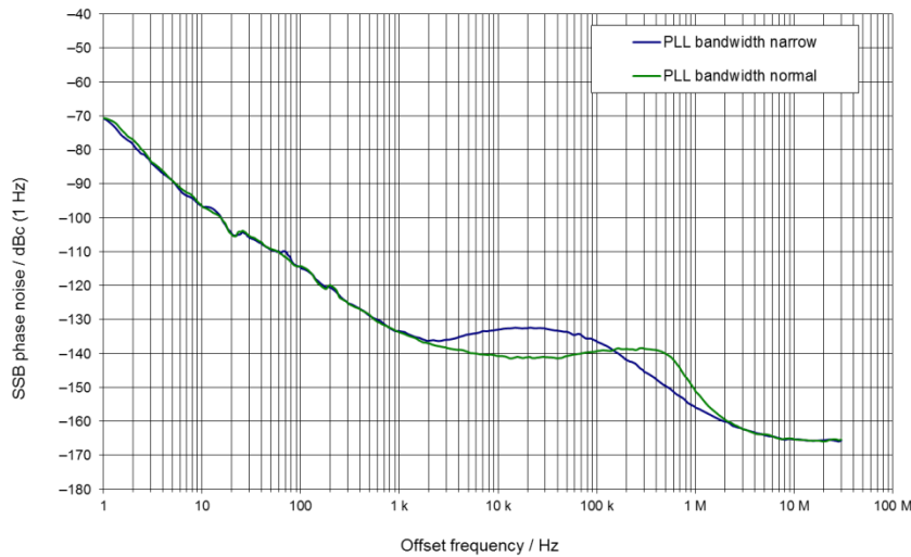
Measured SSB phase noise, f = 1 \text{ GHz} (with R&S ® SMA-B22 enhanced phase noise performance and FM/φM modulator option), comparison of PLL bandwidth normal and narrow (only available for f \leq 3 \text{ GHz} ).
